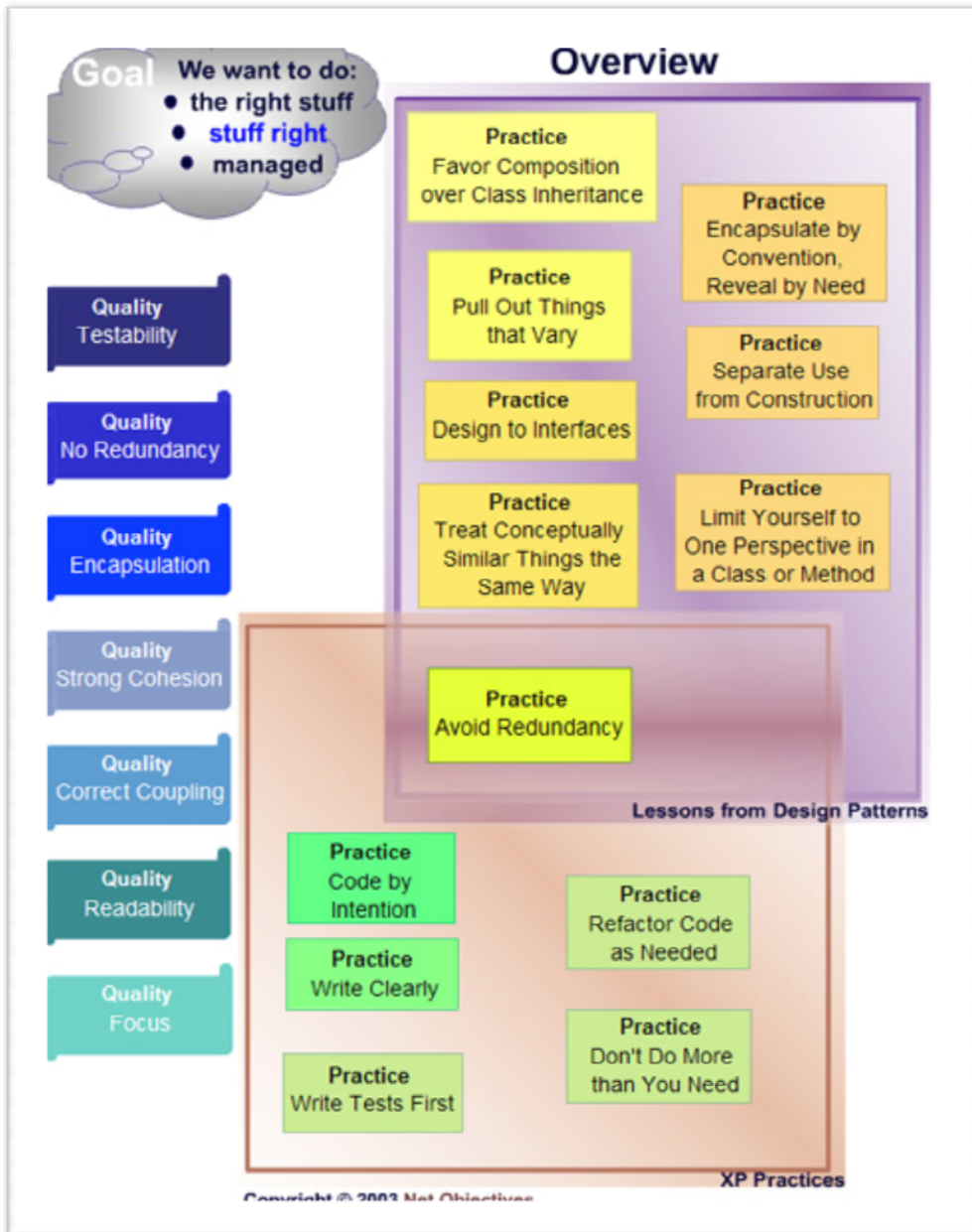
Figure 1: The Thirteen Code Quality Practices
