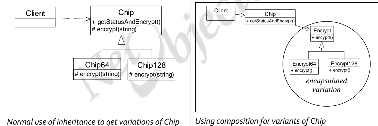
Figure 2: Composition and Encapsulation
